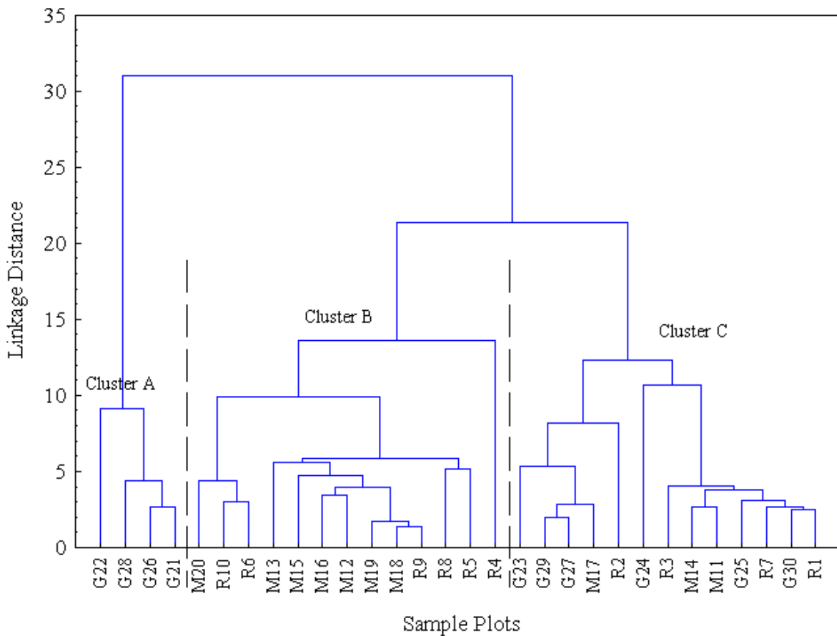
Fig. 4. Hierarchical Cluster Analysis (HCA) dendrogram showing classification of sample plots into three (3) clusters based on species abundance data from the 30 sample plots in Androstachys johnsonii woodland in Gonarezhou National Park (GNP), southeast Zimbabwe. Notes: R-denotes sample plots from the Rhyolite derived soils; M-denotes sample plots from Malvernian bed derived soils and G-denotes sample plots from Granophyre derived soils.
